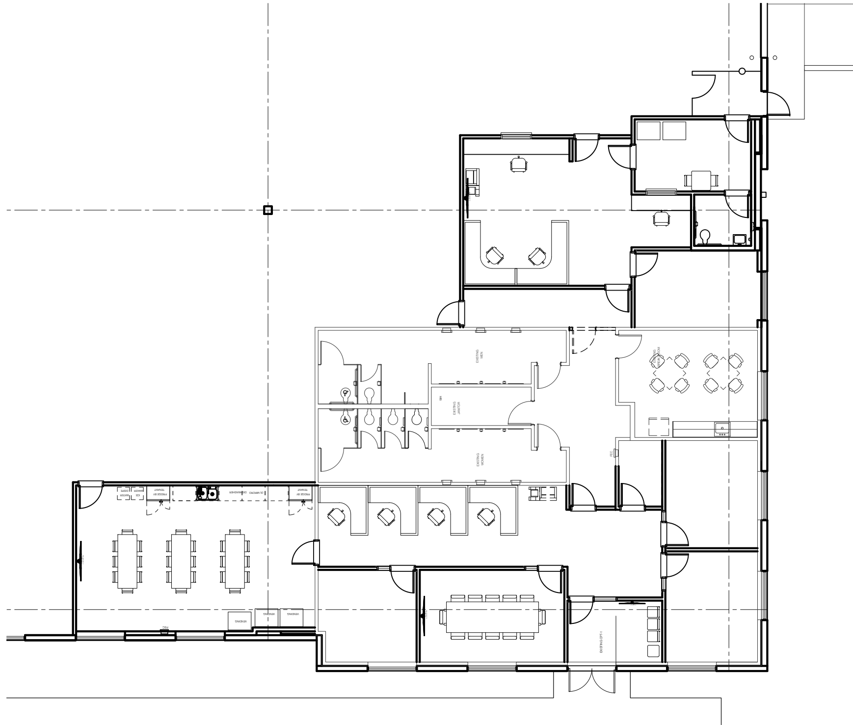
MAIN OFFICE 4,336 SF SCALE: \frac{1}{16}'' = 1'-0''
